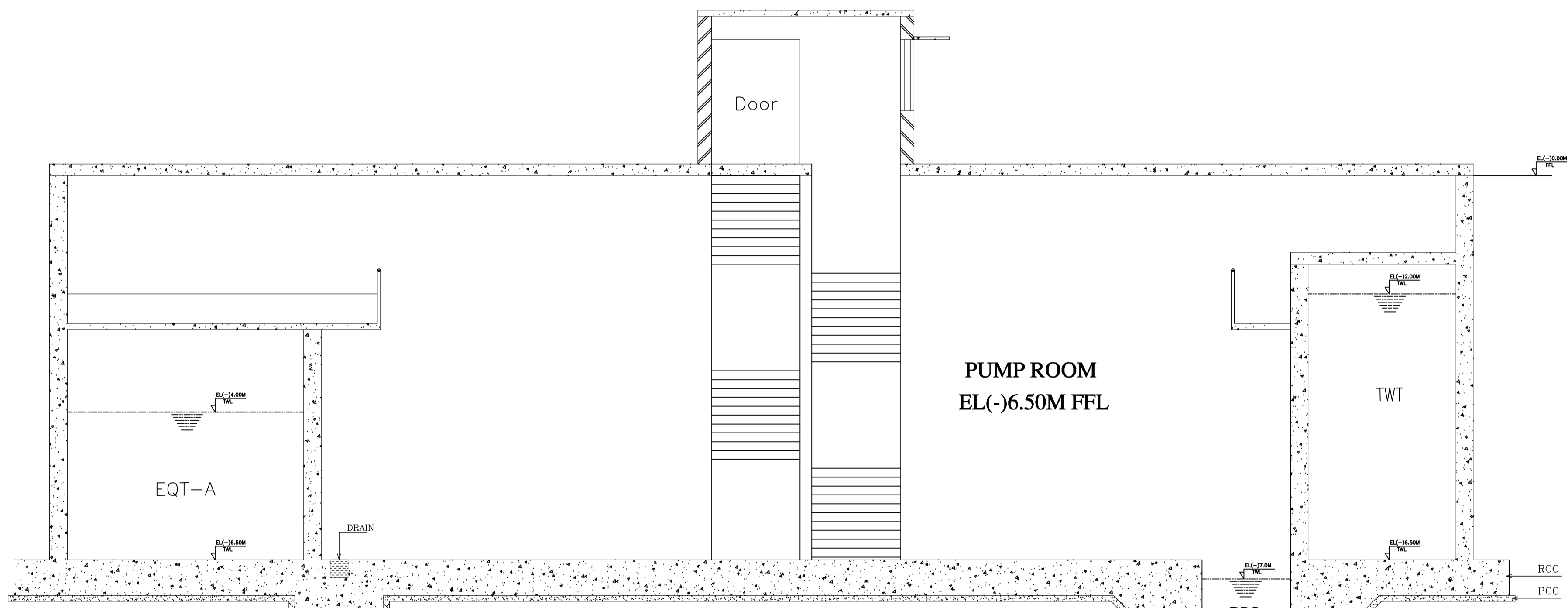
SECTION (B-B)
