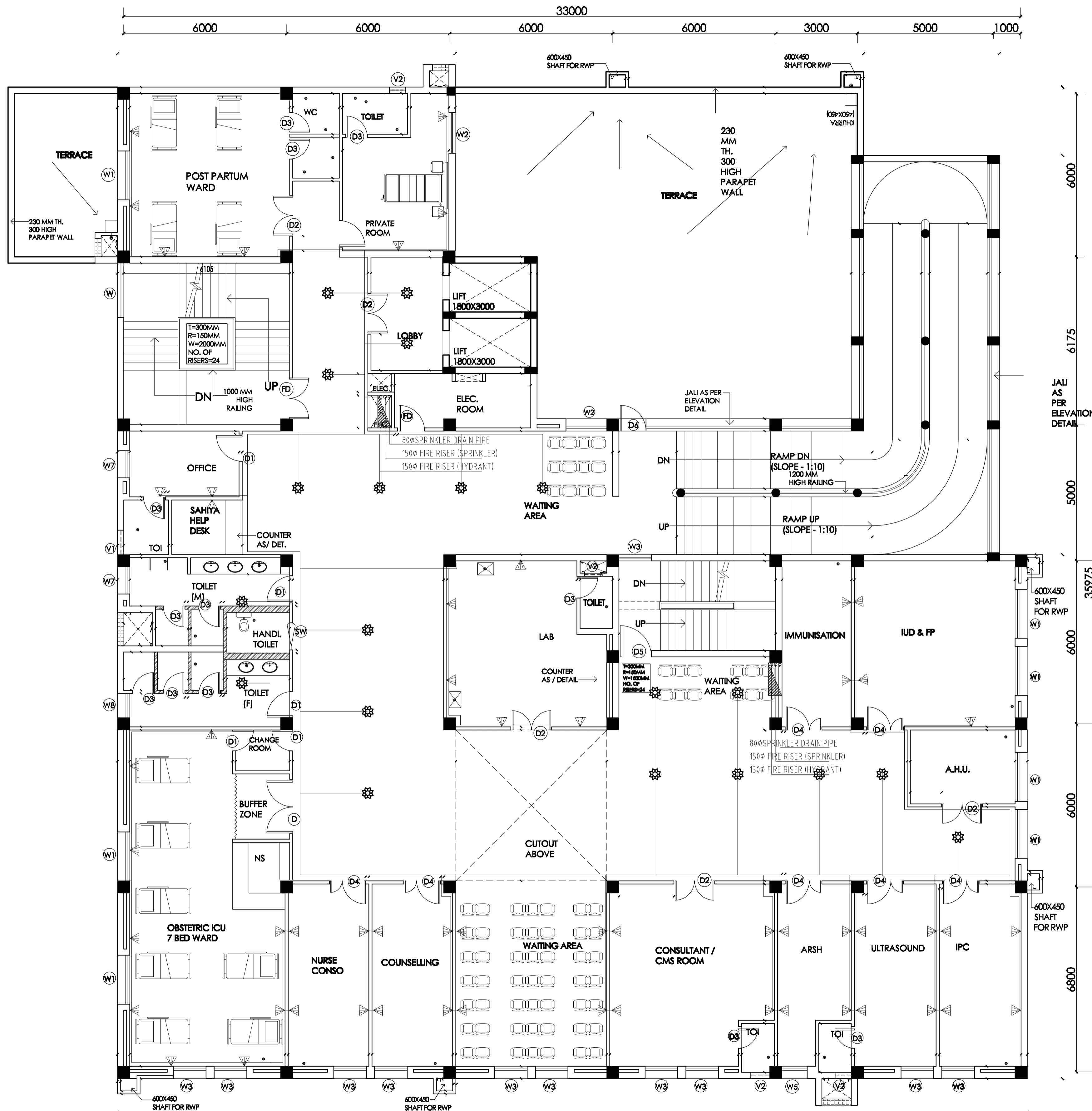
FIRST FLOOR PLAN OPD + OBSTETRIC ICU PRIVATE ROOM - 1 BED
