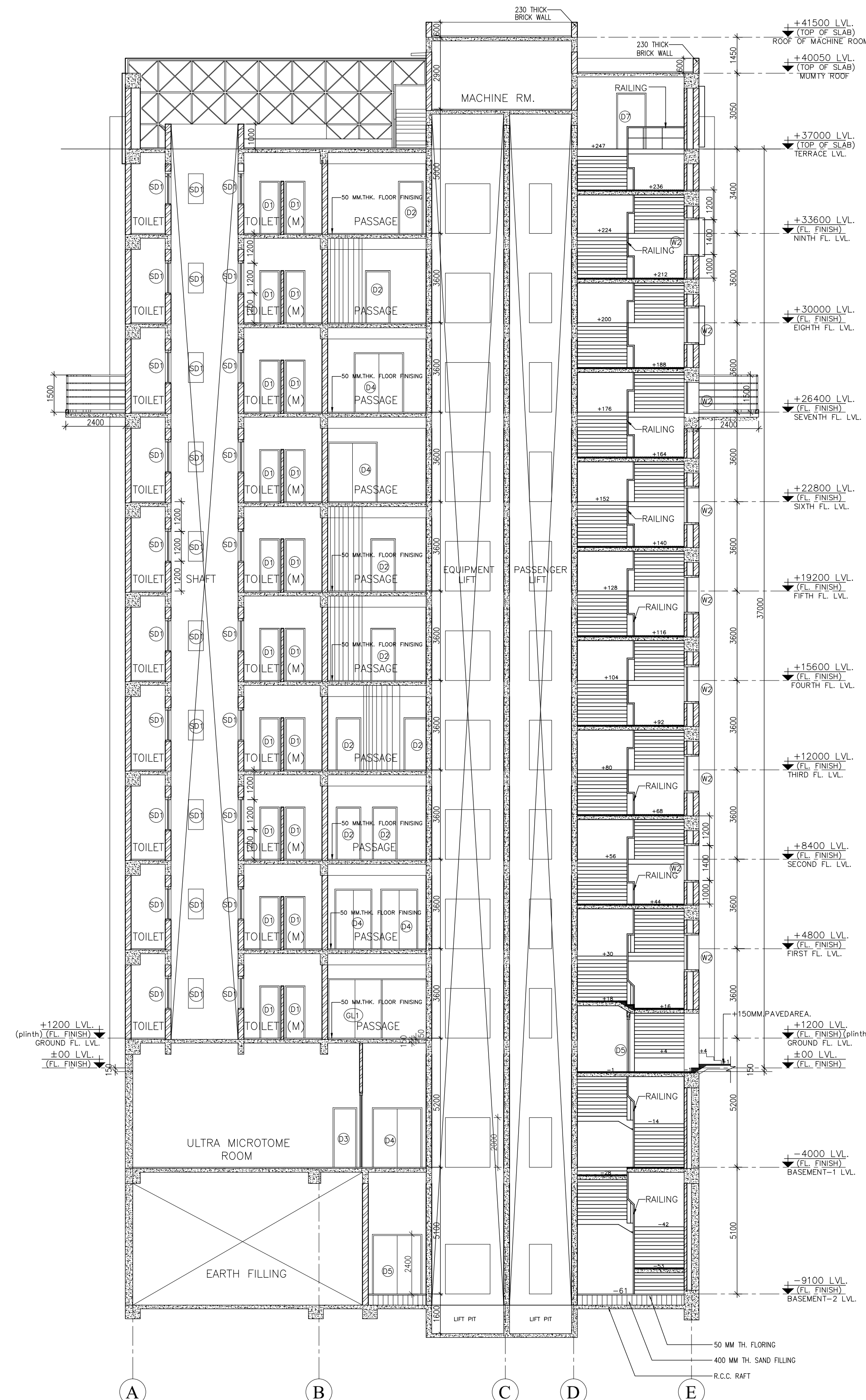
SECTION S2
